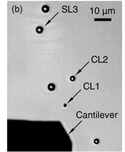
Surface Forces
